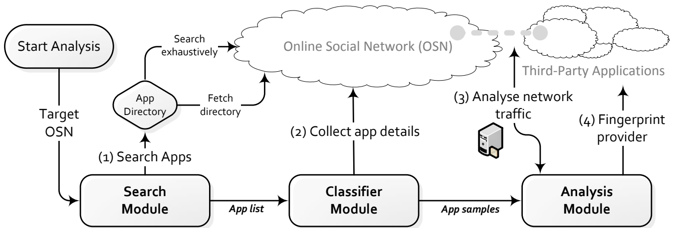
Figure 2: AppInspect, a framework for automated security and privacy analysis of social network ecosystems
