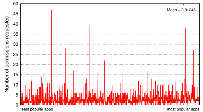
Figure 4: Number of requested permissions for 1,646 application providers
