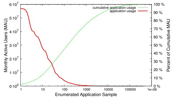
Figure 3: Active monthly users in our sample of 434,687 enumerated applications
